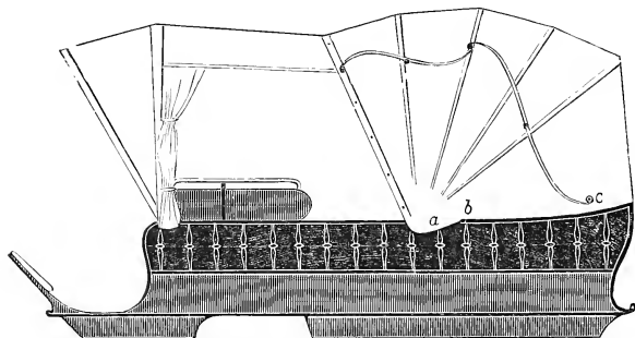
EXTENSION HEAD FOR CARRIAGE.
